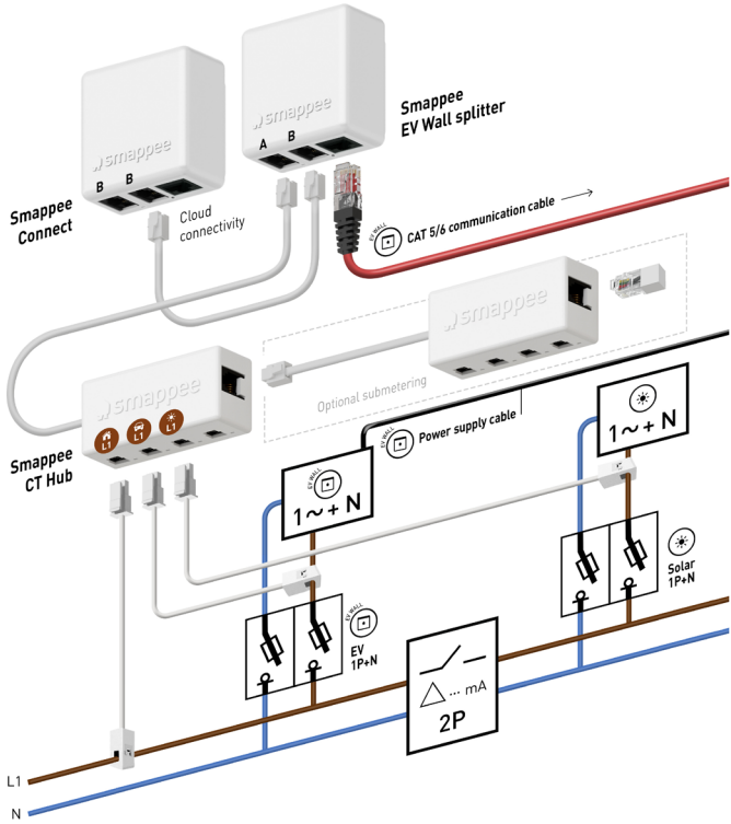
EV Wall single phase connection diagram.
