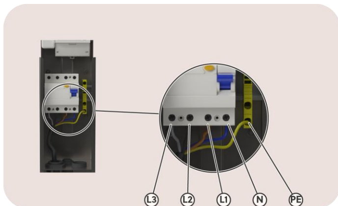
Image 15: View on the power supply connection
