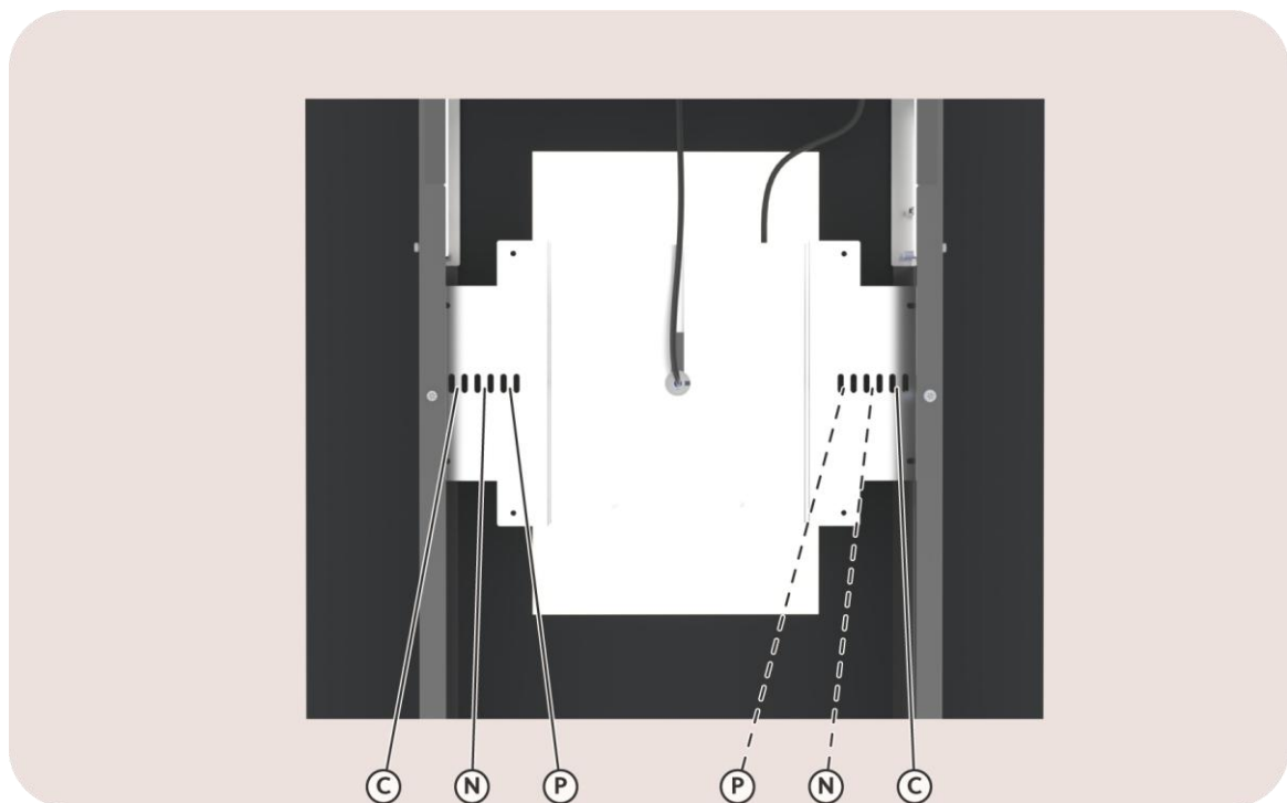
Image 35: View on the attachment of the power supply cable (P), charging cable (C) and network cable (N)
