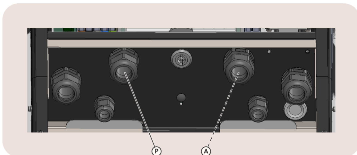
Image 30: View on the cable glands for power supply (P) and optional second power supply (A).
