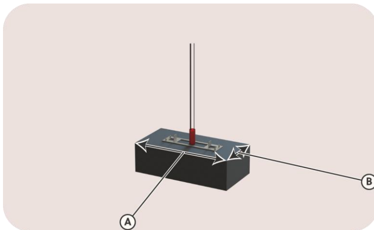
Image 12: View on the minimum dimensions: A \times B = 0.80 \text{ m} \times 0.35 \text{ m} or 2.62 \text{ ft} \times 1.15 \text{ ft}
