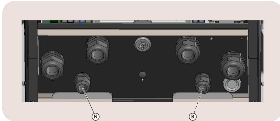
Image 40: View on the cable glands for the network cable (N) and optional cable (B) for daisy-chaining
