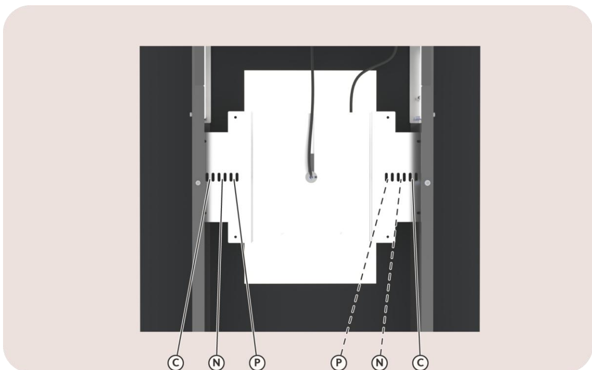
Image 39: View on the attachment of the power supply cable (P), charging cable (C) and network cable (N)
