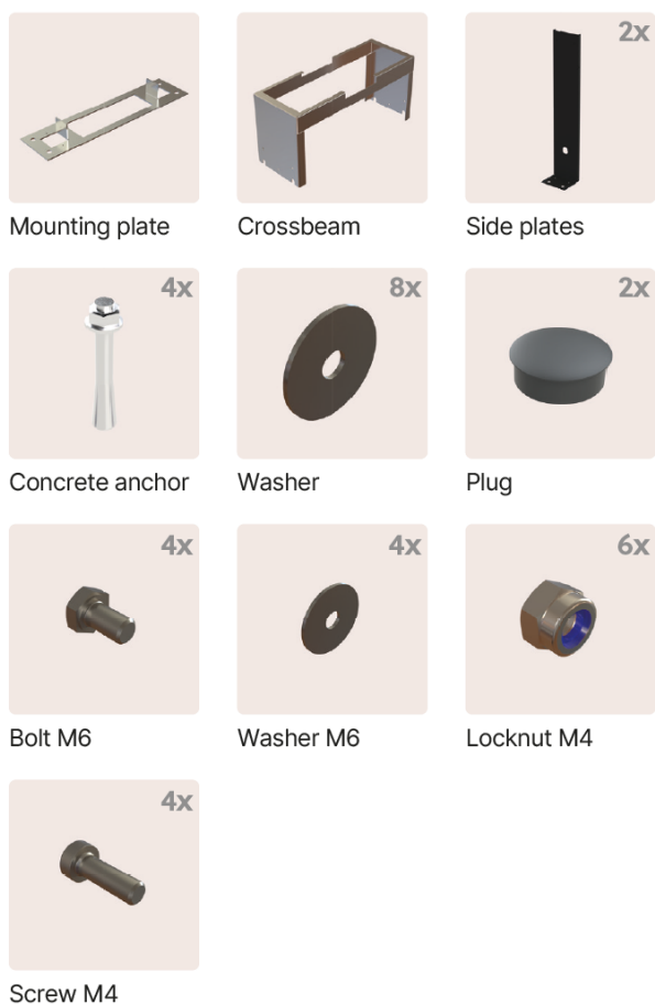
Image 2: Content of the box with the pedestal
