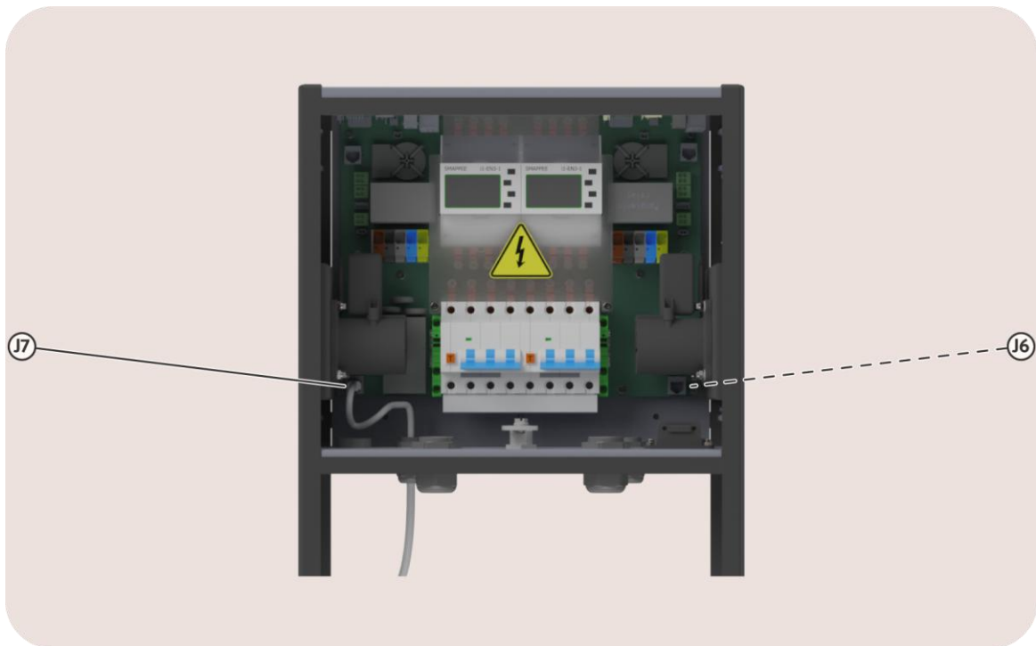
Image 38: View on the port J7 for internet input and the port J6 for optional daisy-chaining
