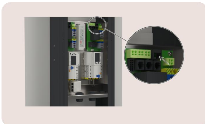
Image 17: View on the A+B port of the relay board
