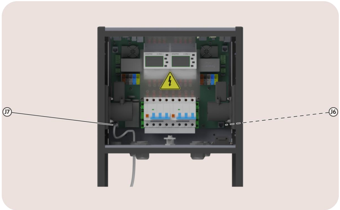
Image 38: View on the port J7 for internet input and the port J6 for optional daisy-chaining
