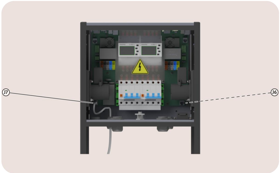
Image 36: View on the port J7 for internet input and the port J6 for optional daisy-chaining
