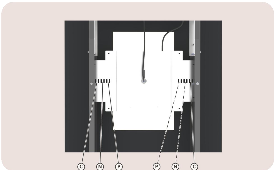
Image 39: View on the attachment of the power supply cable (P), charging cable (C) and network cable (N)
