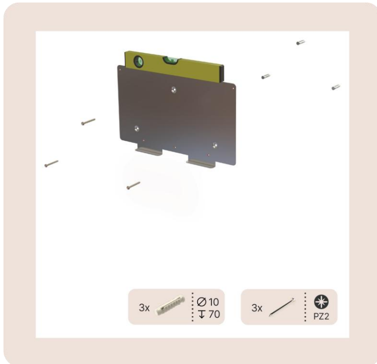
Image 23: View on the wall mounting plate (A) and a spirit level (B)
