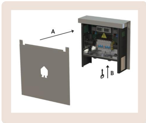
Image 41: View on the EV Dual Wall
