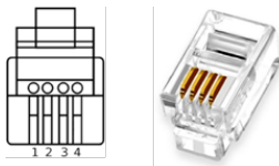
Image 16: Connector
